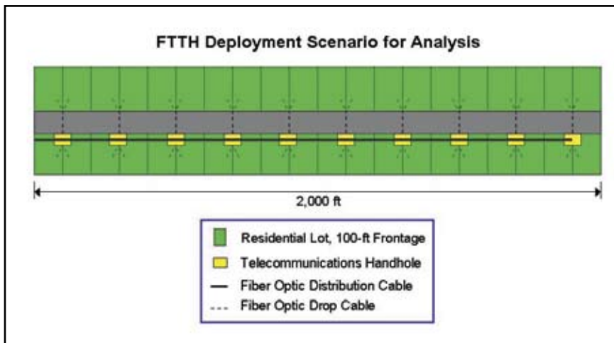
Figure 3: FTTH distribution area for deployment comparison analysis – 2000-foot run serving 40 homes, with 4 homes per network access point.
