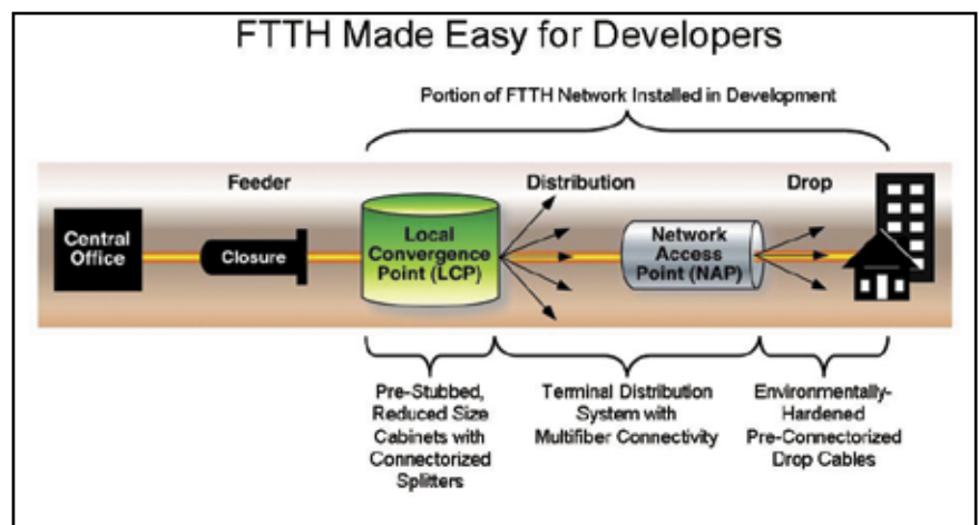
Figure 1: Advanced outside plant FTTH technologies make deployment now easier than ever. This article looks specifically at the portion of the network installed within the development. Usually, this part starts at the local convergence point, where pre-stubbed, reduced-size cabinets with pre-connectorized splitters are installed. It ends with environmentally hardened, pre-connectorized drop cables at users' dwellings. The area between LCP and the drop is the Terminal Distribution System.
